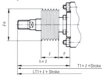
With Single Rod Boot
